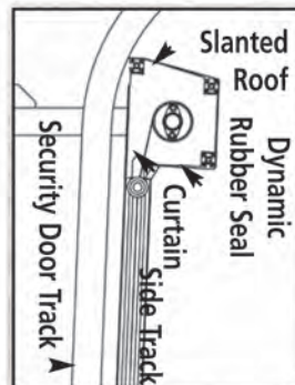
Projection Mount
