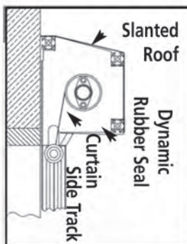
Face Mount
