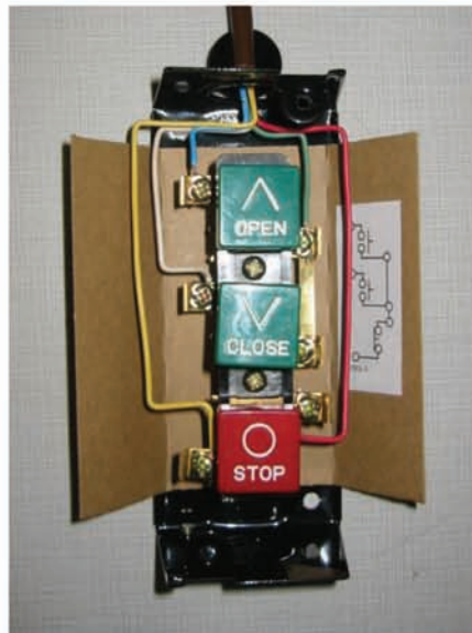
Photo #38 (NEMA-1 Station Wiring)
