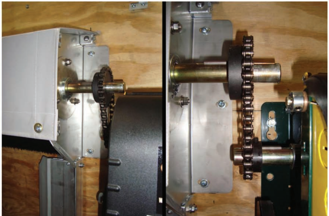
Photo #12 (Chain Installation)
