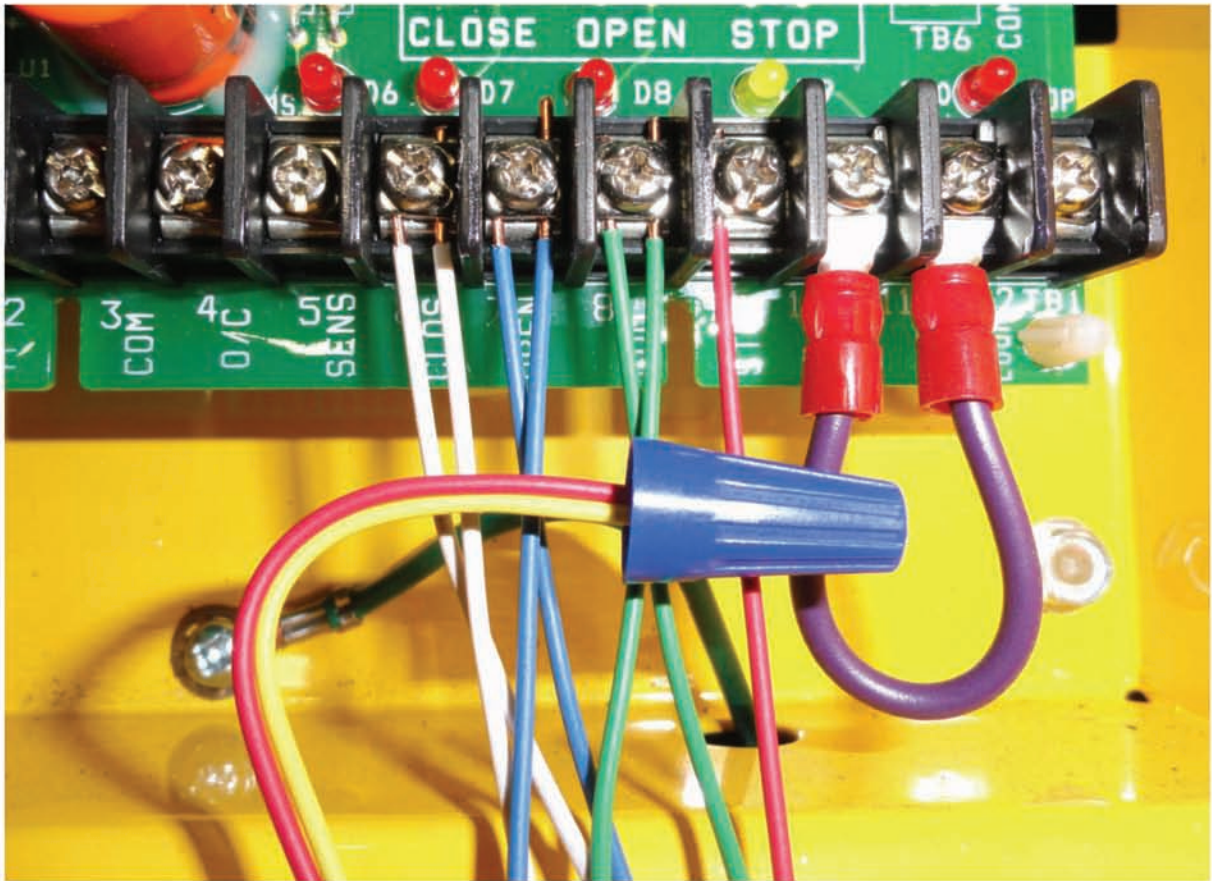
Photo #39 (Additional Station Operator Wiring)
