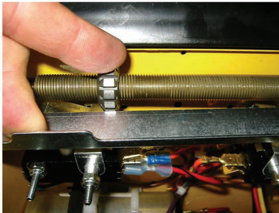
Photo #16 (End Stop Locking Bar)
