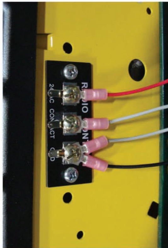
Photo #31 (RF Receiver Wiring)
