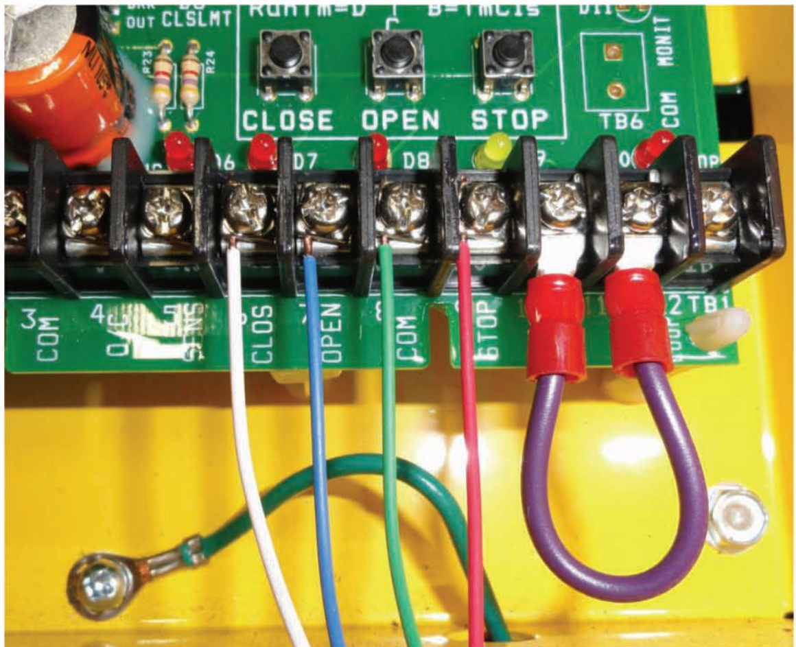
Photo #20 (Operator Control Connections)
