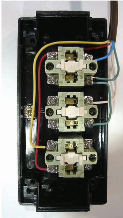
Photo #35 (NEMA-4 Station Wiring)
