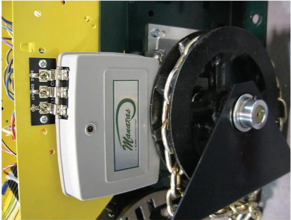
Photo #34 (Manaras Receiver Mounting)
