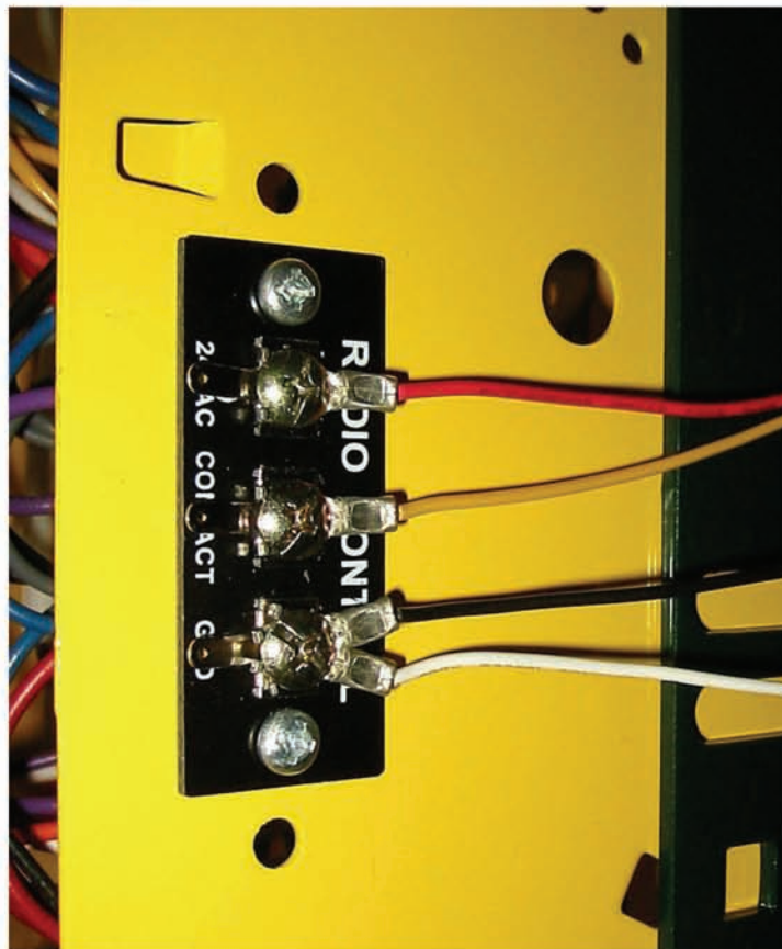
Photo #30 (RF Receiver Wiring)
