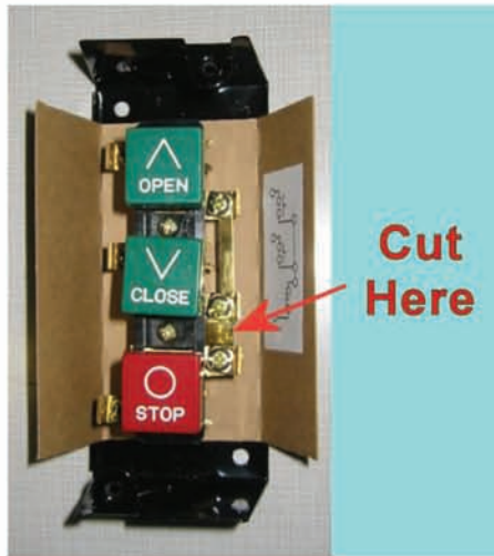
Photo #37 (NEMA-1 Station Cut Point)
