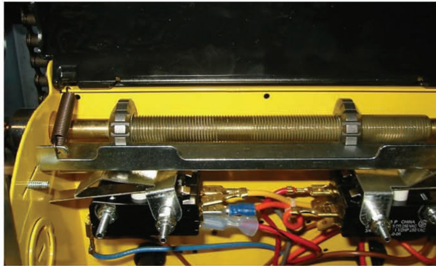
Photo #17 (End Stop Pre-Sets)
