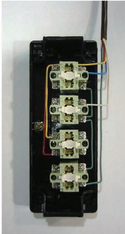
Photo #36 (Locking NEMA-4 Station Wiring)
